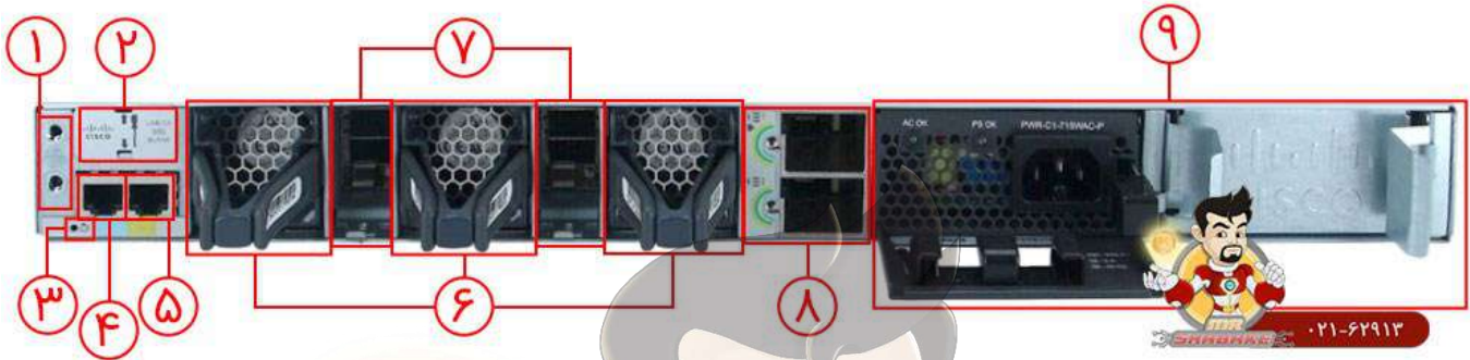
Figure 3 shows the back panel of the C9300-24S-A
